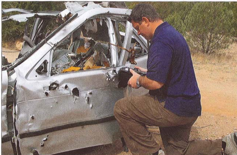
The iris-capture camera on the Cross Match SEEK device has been repurposed to capture images of latent fingerprints in the field. The hood, which is used to block out harsh ambient light when taking iris images, has the same effect when taking images of prints under bright sunlight. Here, images of latent fingerprints are captured on an exploded car using the SEEK II device. www.CrossMatch.com
